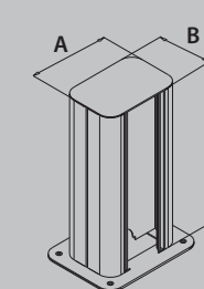
dvostranski stebriček AT-OK 160/110/330
