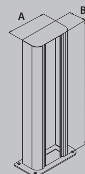
enostranski stebriček AT-OK 160/72/500
